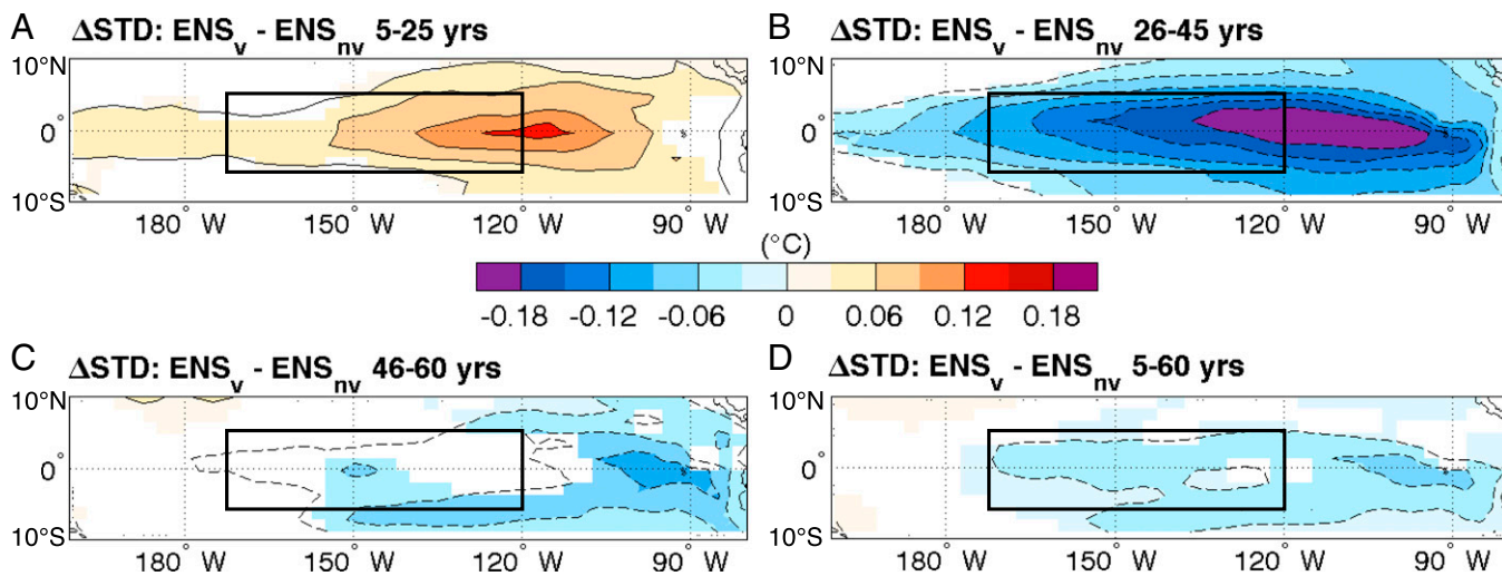
Fig. 2. SST SD changes. Ensemble average change ( ENS_v minus ENS_{nv} ) in the SD of monthly mean SST (in degrees Celsius) for the period 5–25 y (A), 26–45 y (B), and 46–60 y (C) after the eruption and for the entire time series (D). Changes that are significant at the 95% confidence level using an F test are shaded. The contour interval is 0.03 °C (dashed, negative anomalies; solid, positive anomalies; the zero line is omitted). We discard the first 4 y to remove the hemispheric-wide cooling due the eruption. The SD is calculated from the concatenated time series using all 10 members in each ensemble. Hence, 210 y of data are used to calculate the SD in A: 10 members \times 21 y; 200 in B, 150 in C, and 560 y in D. As is commonly done when examining ENSO, we apply a 5-mo running mean on the SST anomalies to damp high-frequency ocean variability unrelated to ENSO. The box shows the Niño-3.4 area.
