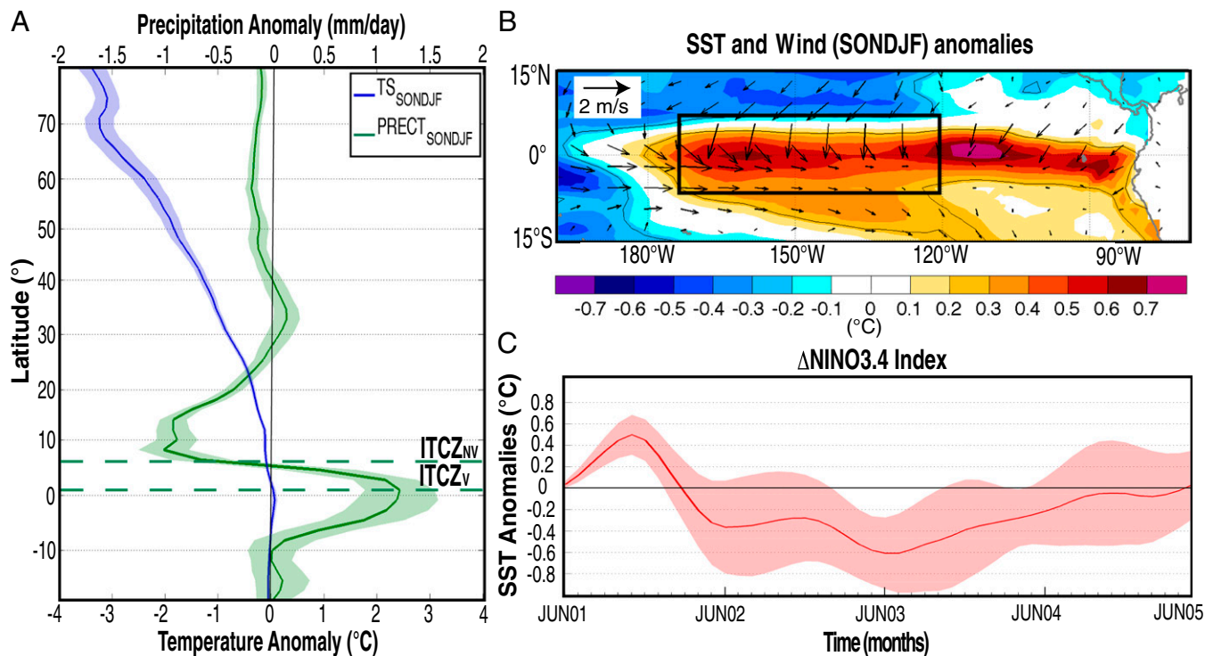
Fig. 1. Temperature, precipitation and wind anomalies following the eruption. (A) Ensemble average change ( ENS_{\text{V}} minus ENS_{\text{NV}} ) in the zonal-mean surface temperature (blue) and precipitation (green) over the Pacific basin (150°E to 90°W), for the period 4–9 mo following the start of the eruption (September to February). Shading shows the approximate 95% confidence intervals (twice the SEM) of the change seen in all 20 pairs of experiments. The bold green dashed lines show the ensemble-averaged position of the ITCZ in the no-volcano and volcano simulations. (B) Ensemble average changes in near-surface wind (arrows) and SST (shading) 4–9 mo following the start of the eruption. The box shows the Niño-3.4 area. The contours delineate the areas where the SST anomalies are significant at the 95% confidence level using a Student t test. (C) Ensemble average changes in Niño-3.4 index due to the eruption.
